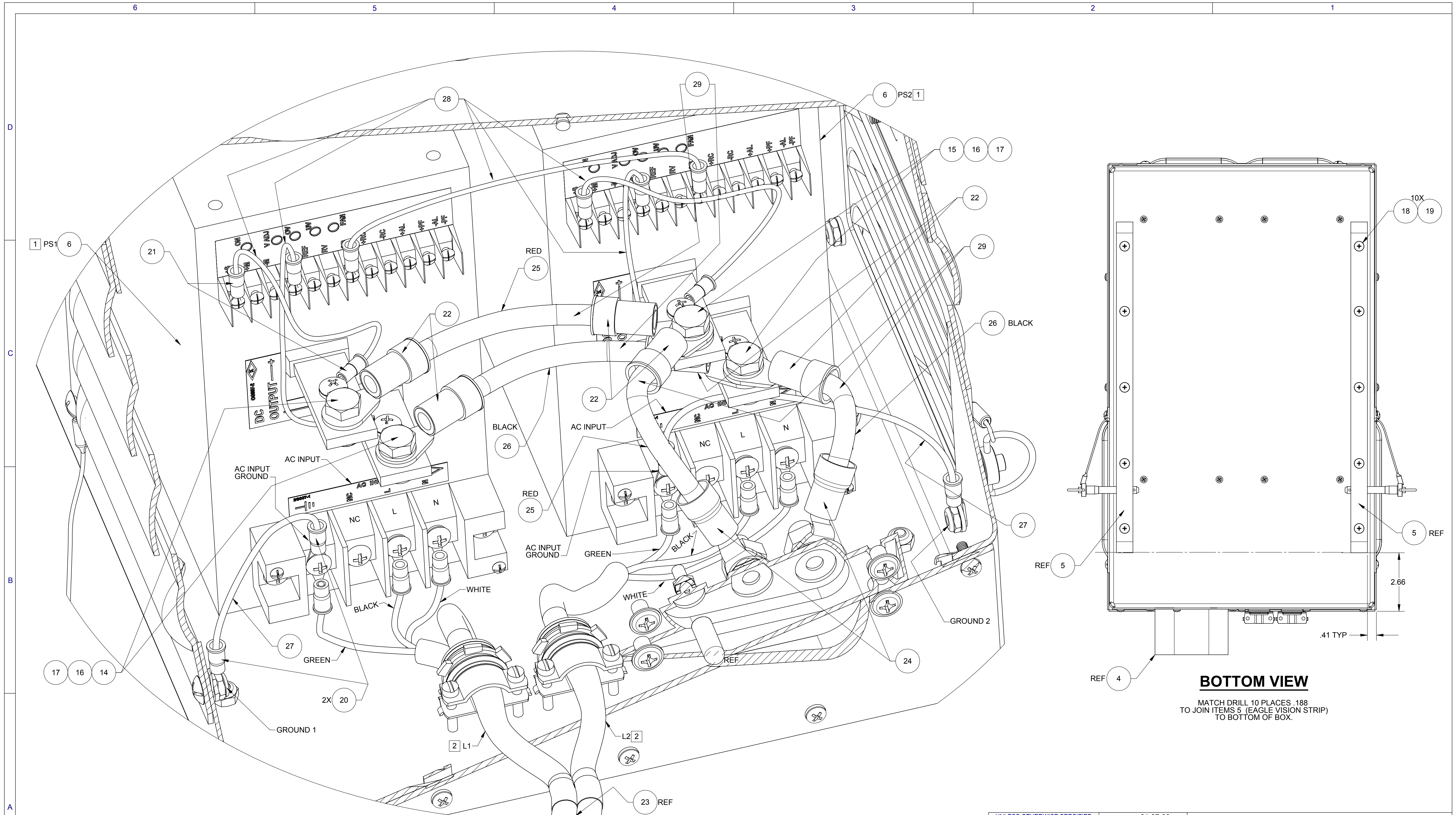
DETAIL A BROKEN-OUT SECTION OF GROUND POWER SUPPLY BOX.
